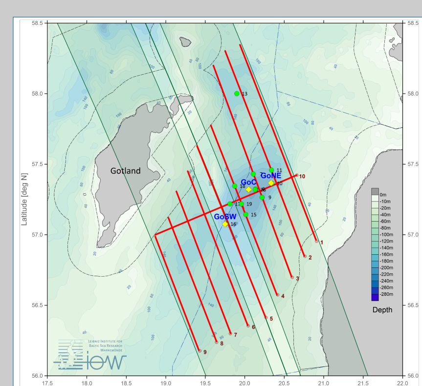
Fig. 6 10 ScanFish tracks in SWOT swath
