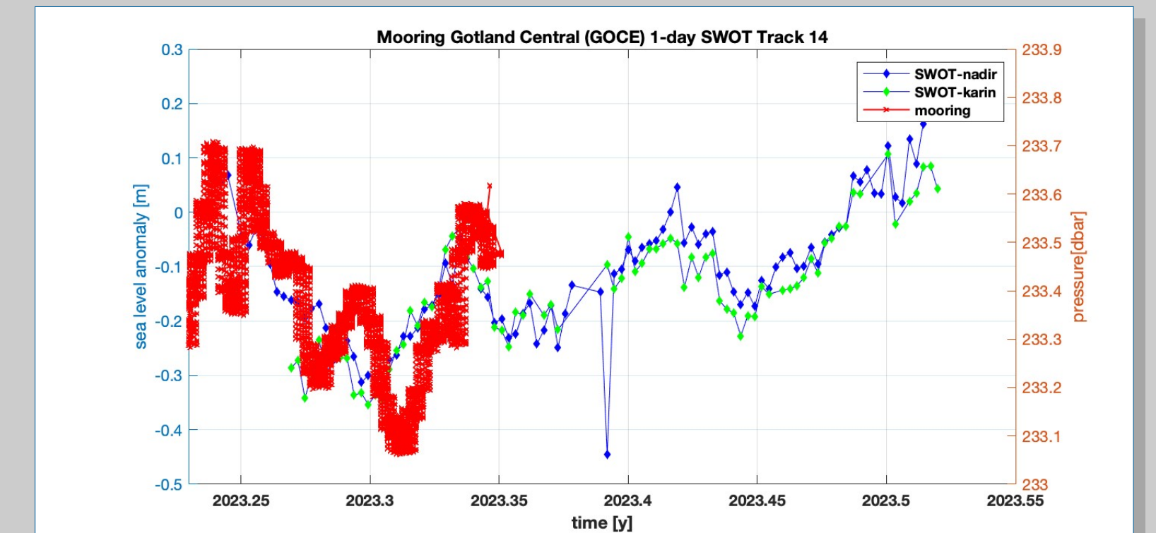
Fig. 10 SWOT-nadir (blue) and SWOT-karin (green) against pressure mooring GOCE-CB
