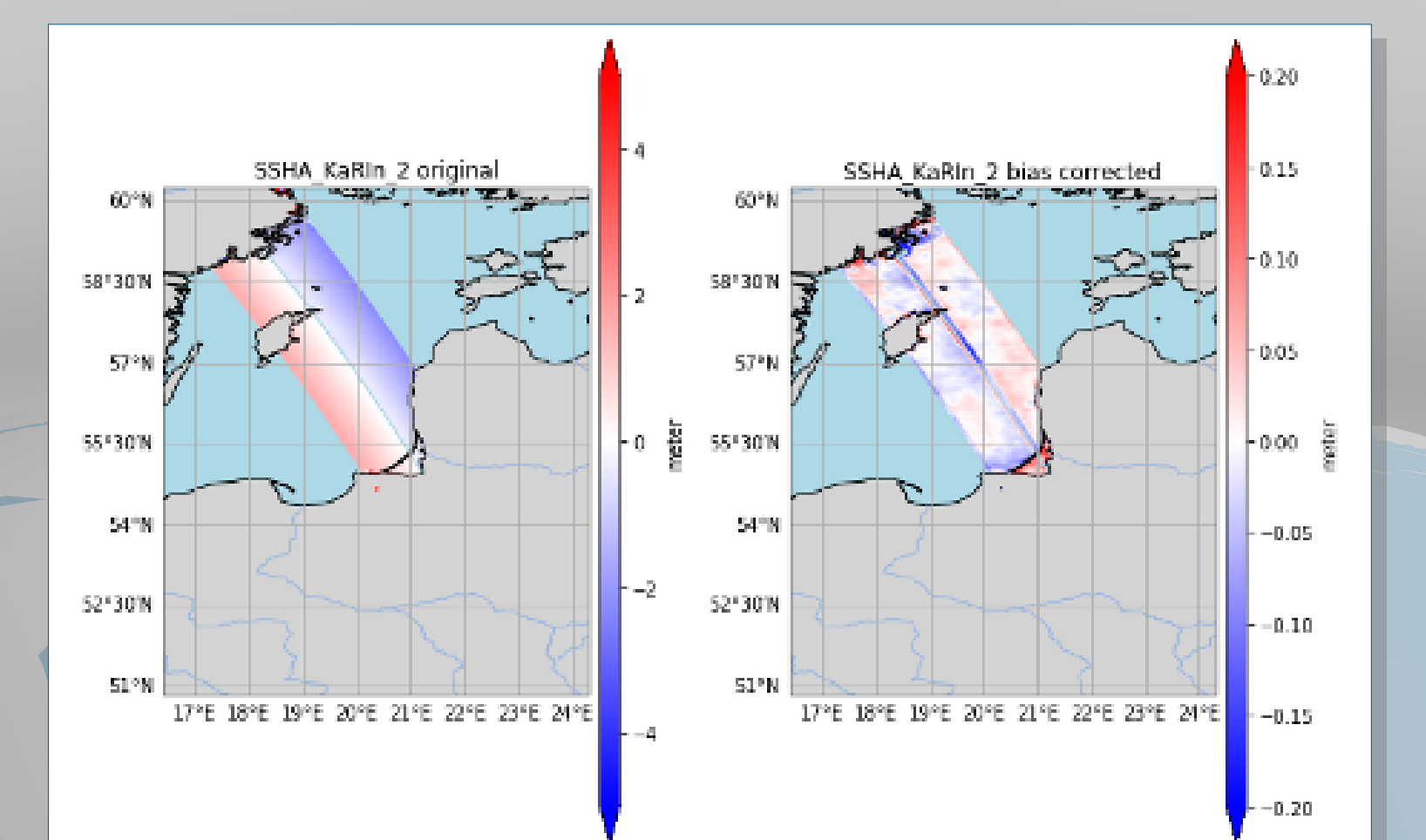
Fig. 13 SWOT-Karin post-processing of L2 data
