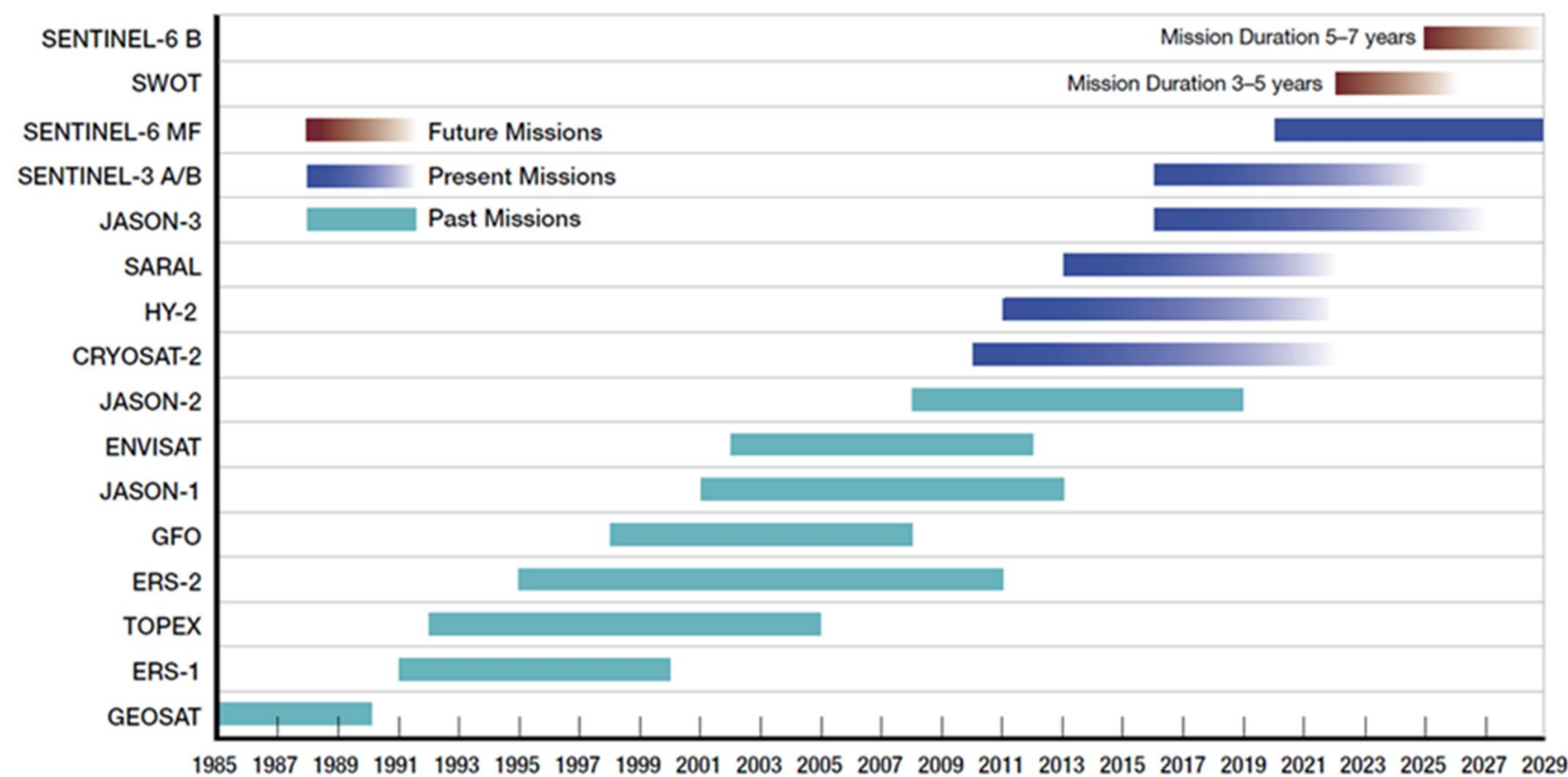
Continuity of Satellite Altimetry Missions over 30+ years
